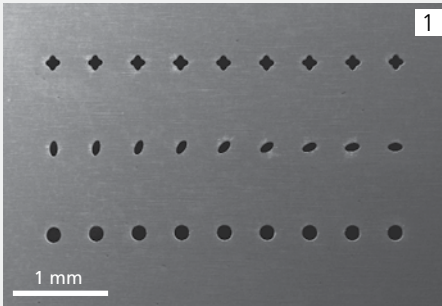
1 Flexible geometries in 300-μm-thick steel (SEM image, exit side)
