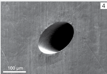
4 Detail of figure 1: Elliptical bore hole, 190 μm long, 110 μm wide (SEM image)
