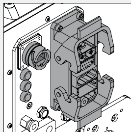
Industry-proven connectors (Ethernet, power, PLC, laser) and status LEDs
