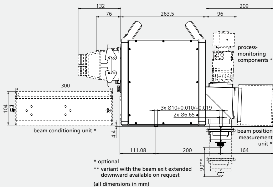
Side view precSYS
