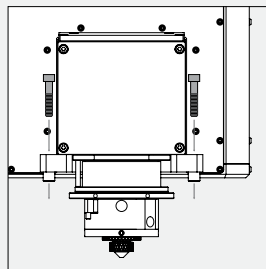
Mounting holes near objective for precise positioning of the beam exit (3-point support)
