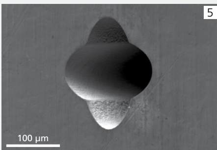
5 Detail of figure 1: Geometric flexibility achieved by two overlapping ellipses 190 μm long and 110 μm wide, each (SEM image)
