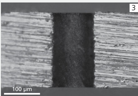
3 Cross section of a 100-μm bore hole in 200-μm thick steel with perpendicular wall contour (zero taper), process time 1 s
