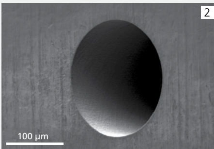
2 Ideally-formed round single bore hole with 200 μm diameter from figure 1 magnified (SEM image)
